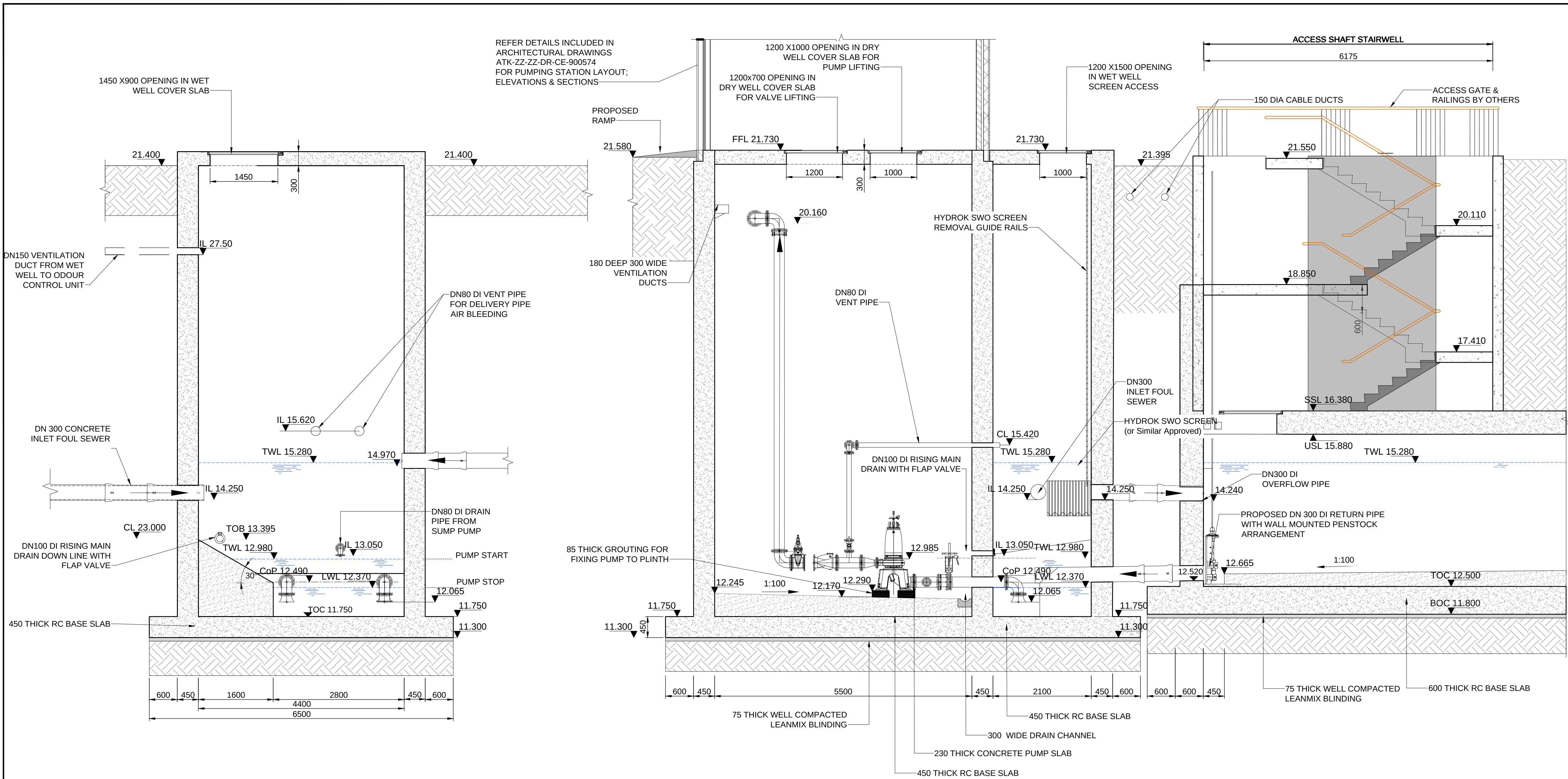
B SECTION 900572 SCALE 1:50
