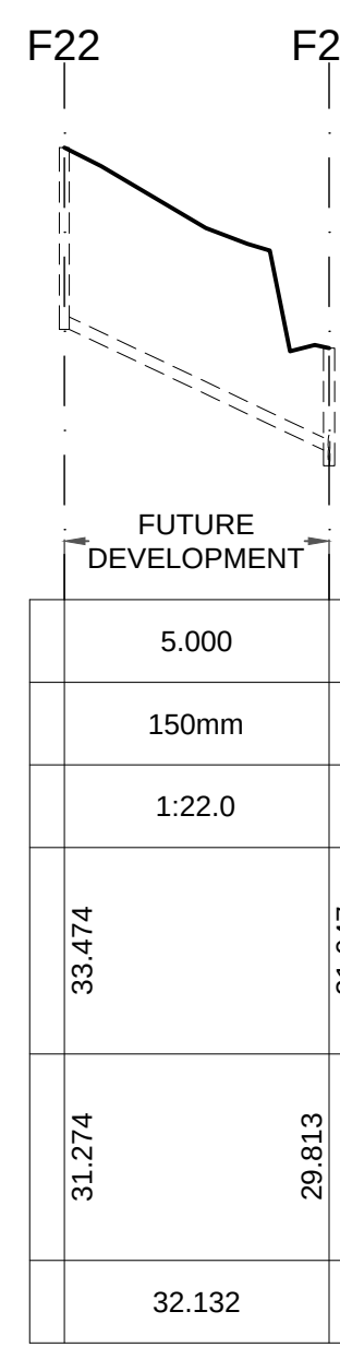
Link Name Section Type Slope (1:X) Cover Level (m) Invert Level (m) Length (m)
