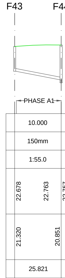
Link Name Section Type Slope (1:X) Cover Level (m) Invert Level (m) Length (m)
