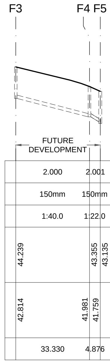
Link Name Section Type Slope (1:X) Cover Level (m) Invert Level (m) Length (m)
