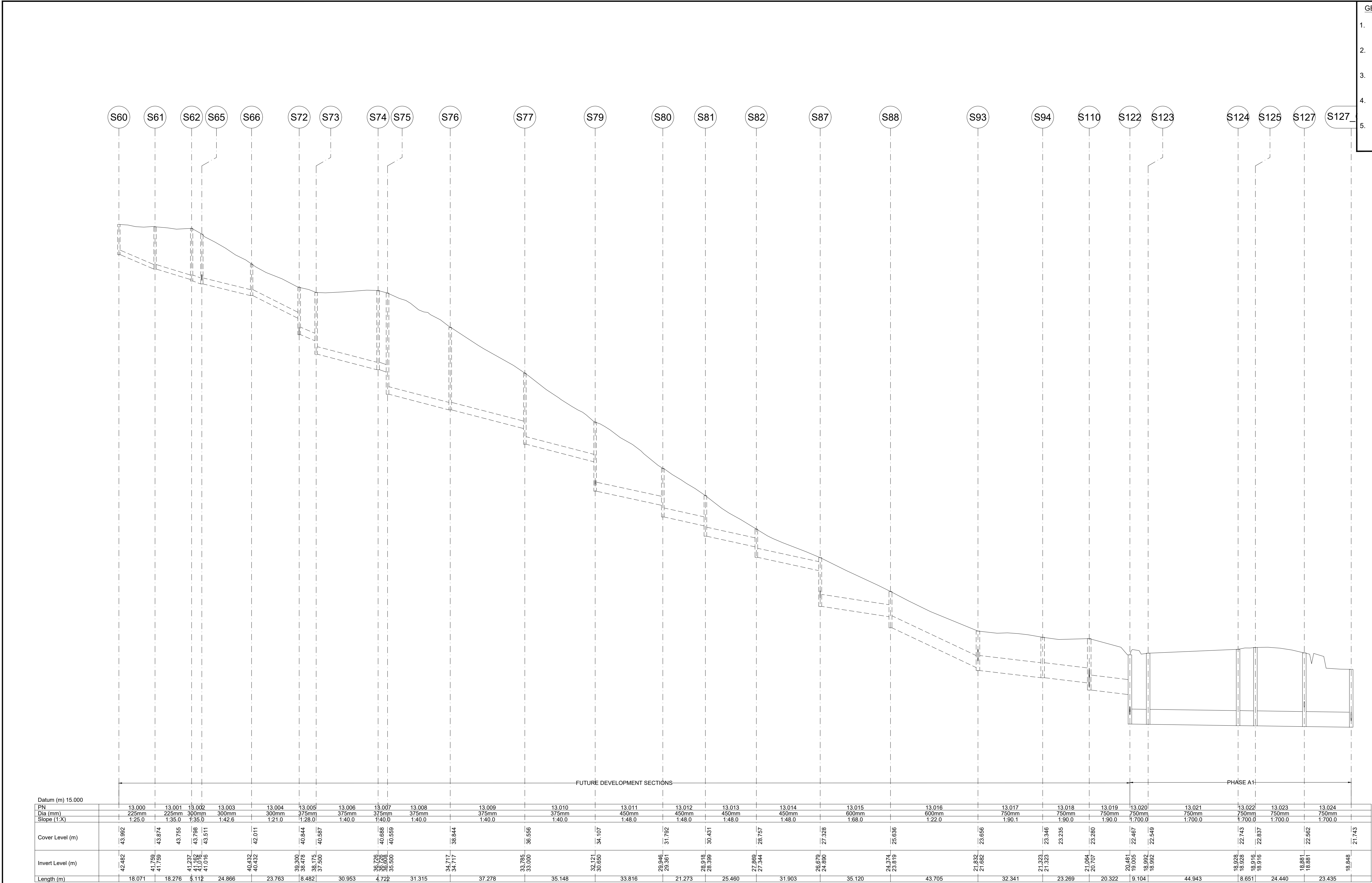
Longitudinal Section S60 - S127_OUT Scale 1:1000 (Horizontally), 1:100 (Vertically)
