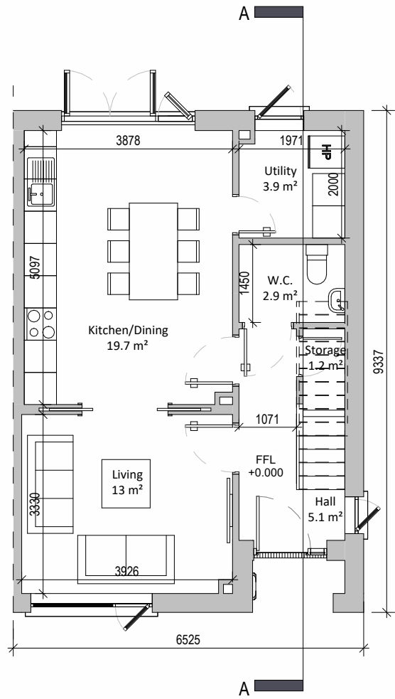
① Ground Floor Plan 1 : 100
