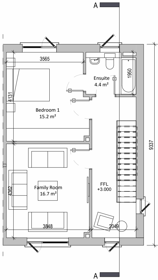
② First Floor Plan 1 : 100
