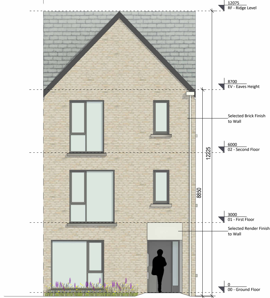
④ Front Elevation 1 : 100
