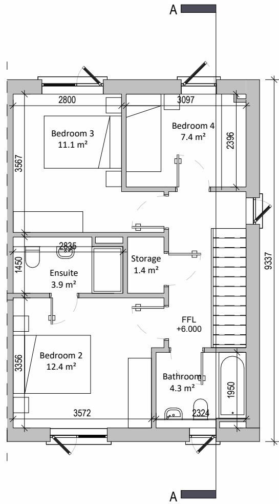
③ Second Floor Plan 1 : 100
