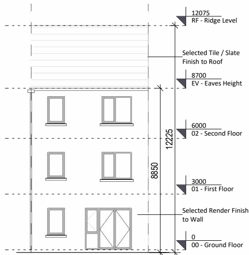
⑤ Rear Elevation 1 : 200
