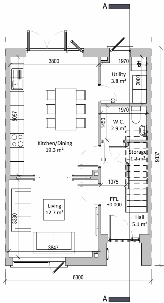
① Ground Floor Plan 1 : 100
