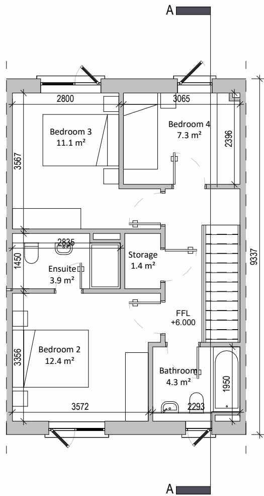
③ Second Floor Plan 1 : 100
