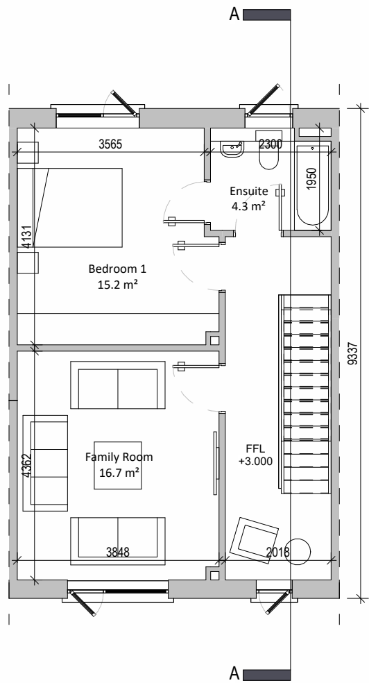
② First Floor Plan 1 : 100
