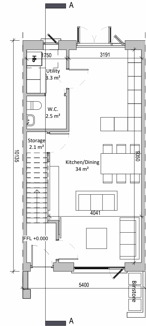
1 Ground Floor Plan 1 : 100
