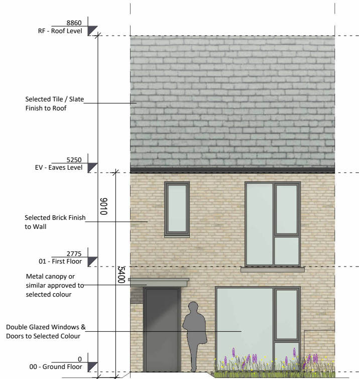
3 Front Elevation 1 : 100
