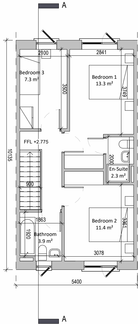
2 First Floor Plan 1 : 100
