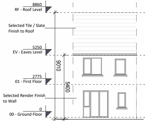
4 Rear Elevation 1 : 200
