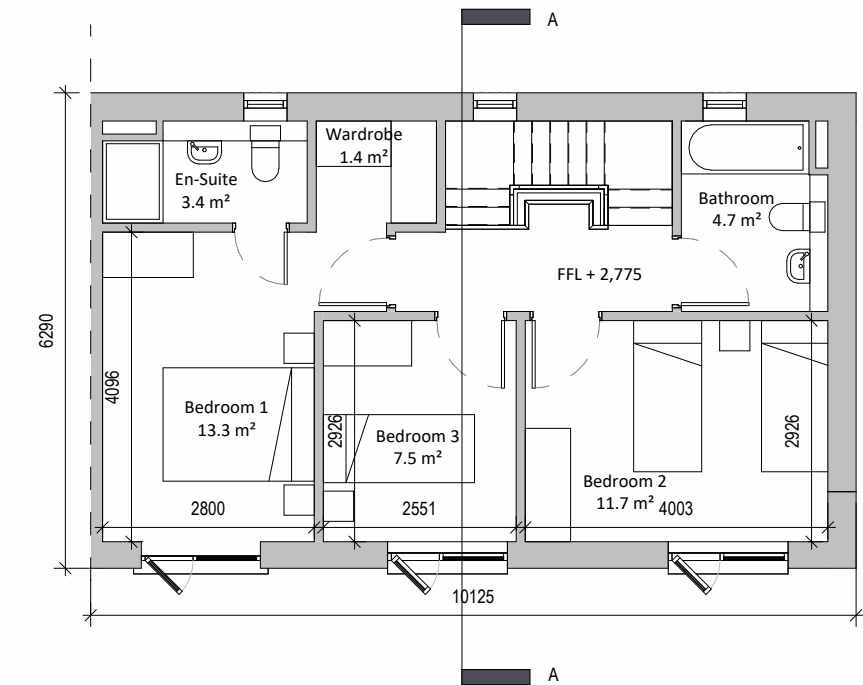
2 First Floor Plan 1 : 100
