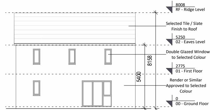
4 Rear Elevation 1 : 200
