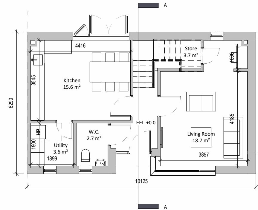
1 Ground Floor Plan 1 : 100
