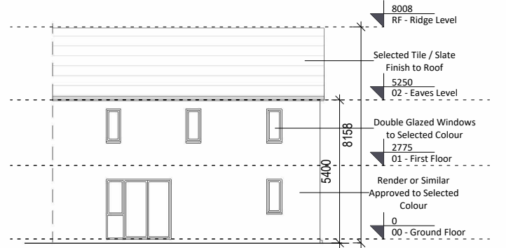
4 Rear Elevation 1 : 200
