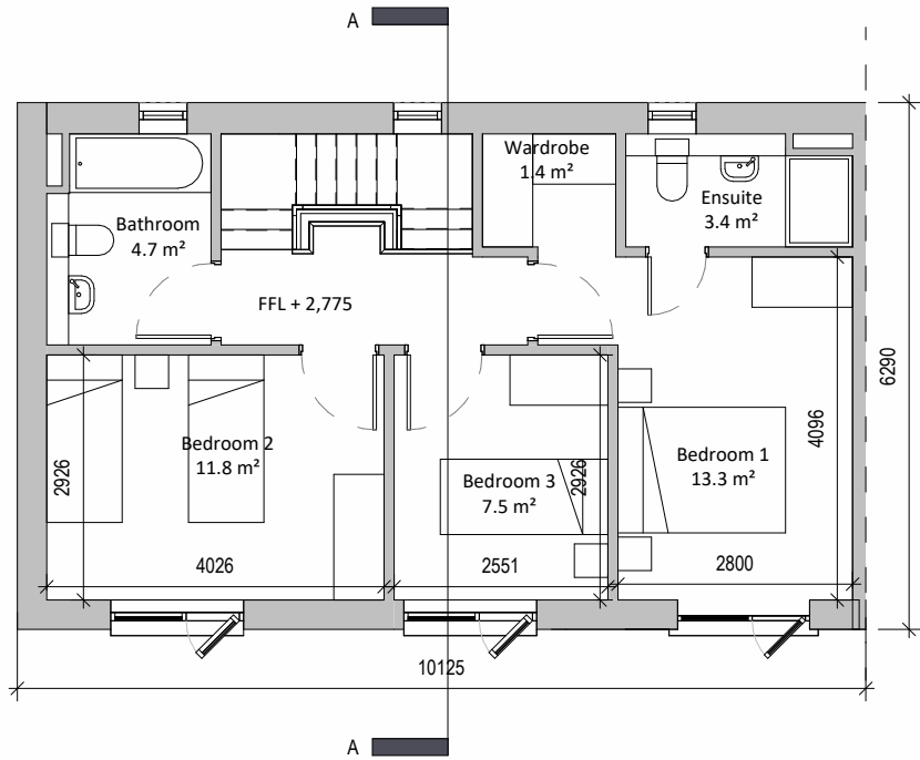
2 First Floor Plan 1 : 100
