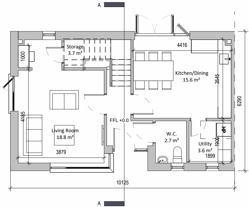
1 Ground Floor Plan 1 : 100
