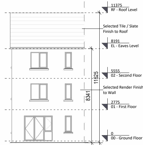
⑤ Rear Elevation 1 : 200
