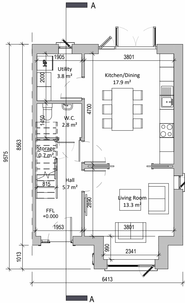
① Ground Floor Plan 1 : 100
