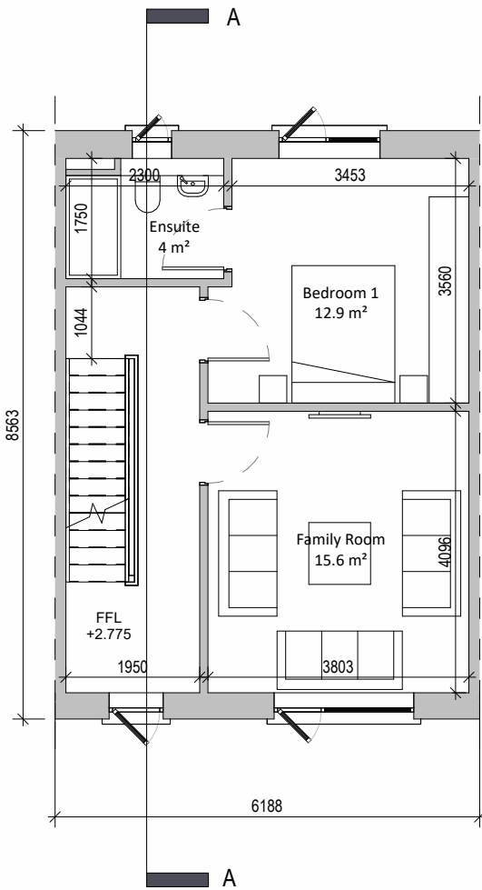
2 First Floor Plan 1 : 100
