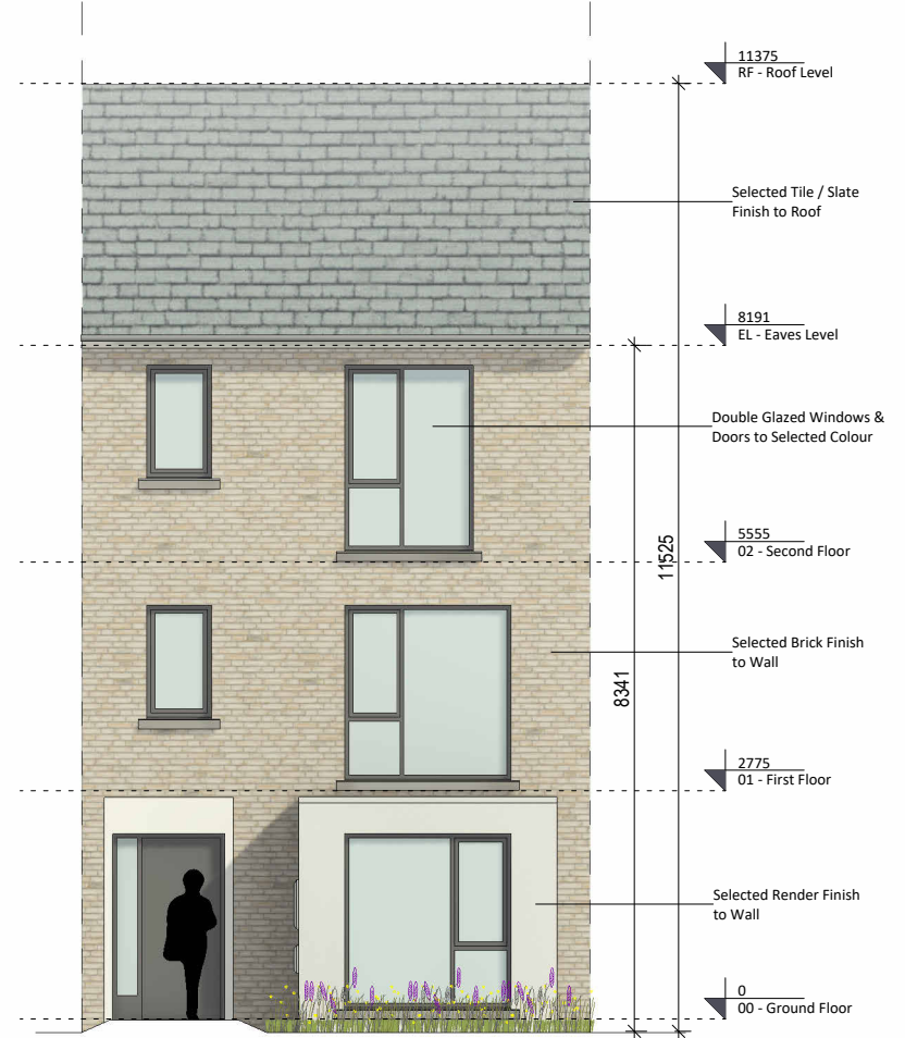
4 Front Elevation 1 : 100
