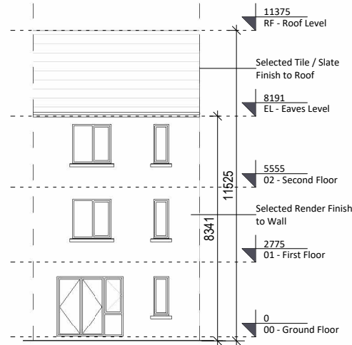
4 Front Elevation 1 : 100
