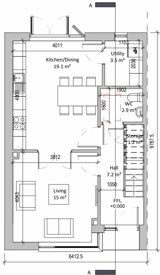
1 Ground Floor Plan 1 : 100
