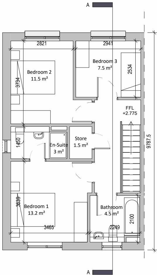
2 First Floor Plan 1 : 100
