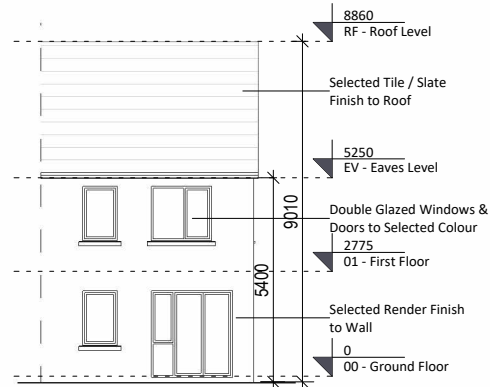
4 Rear Elevation 1 : 200
