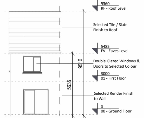
4 Rear Elevation 1 : 200
