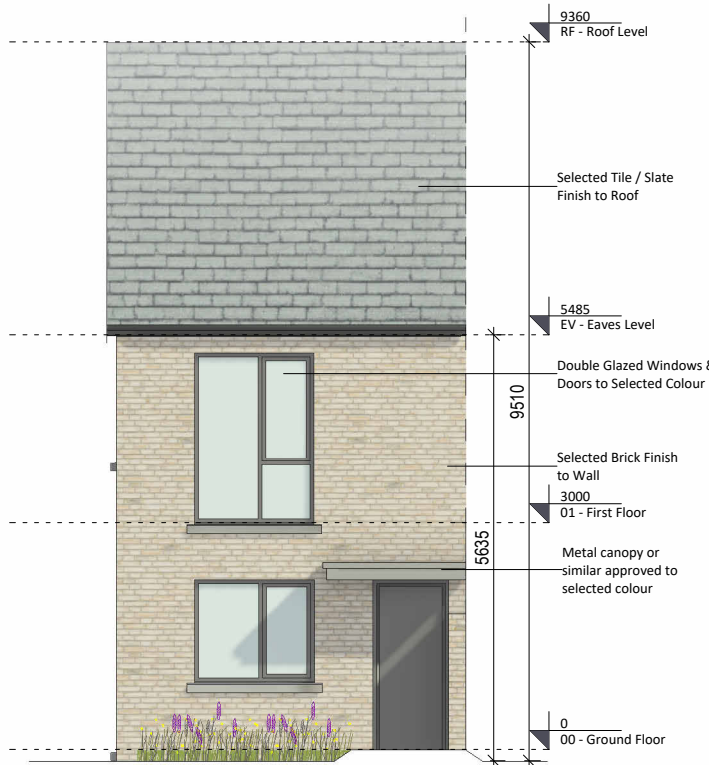
3 Front Elevation 1 : 100
