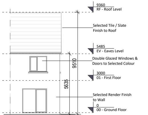
4 Rear Elevation 1 : 200
