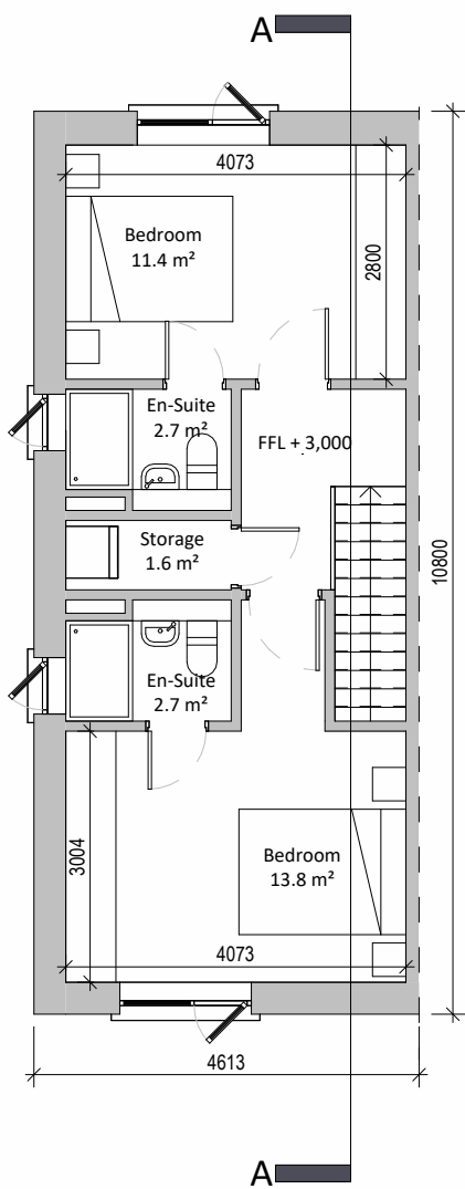
2 First Floor Plan 1 : 100
