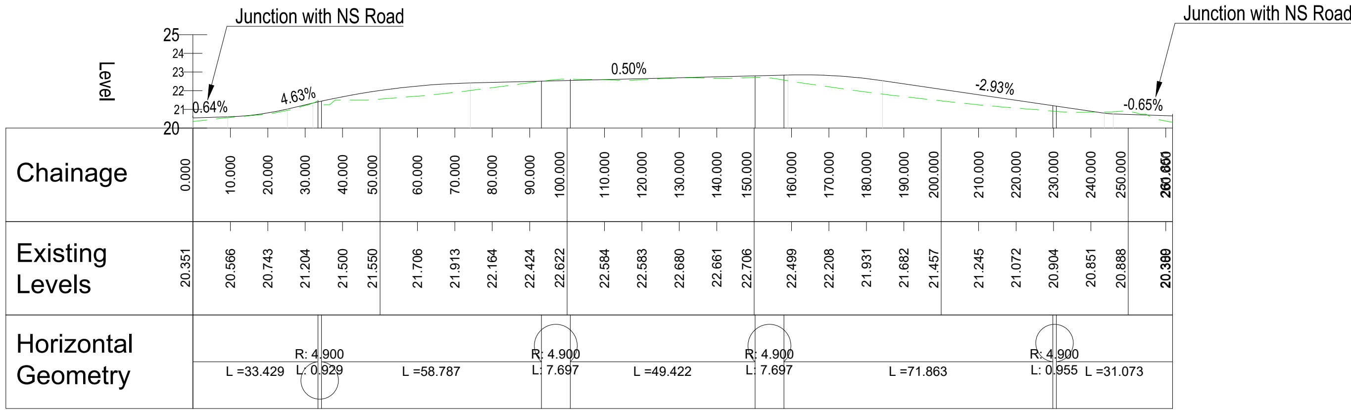
LONGSECTION - ALIGNMENT - PHASE 1 - ROAD 4 SCALE: H 1:1000,V 1:200. DATUM: 20.000
