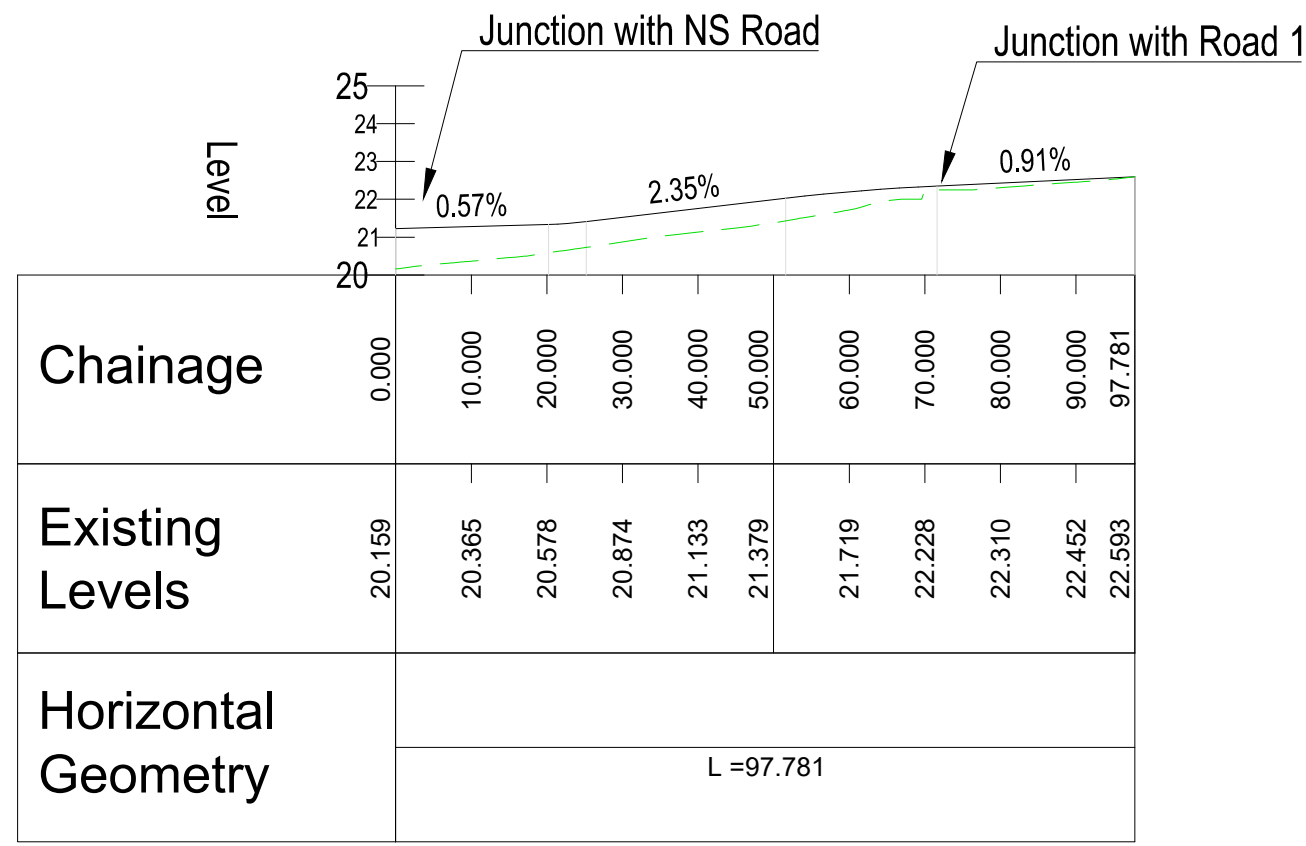
LONGSECTION - ALIGNMENT - PHASE 1 - ROAD 3 SCALE: H 1:1000,V 1:200. DATUM: 20.000
