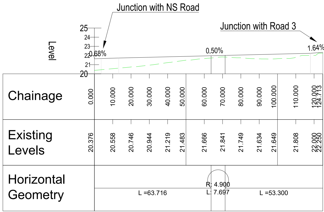
LONGSECTION - ALIGNMENT - PHASE 1 - ROAD 1 SCALE: H 1:1000,V 1:200. DATUM: 20.000
