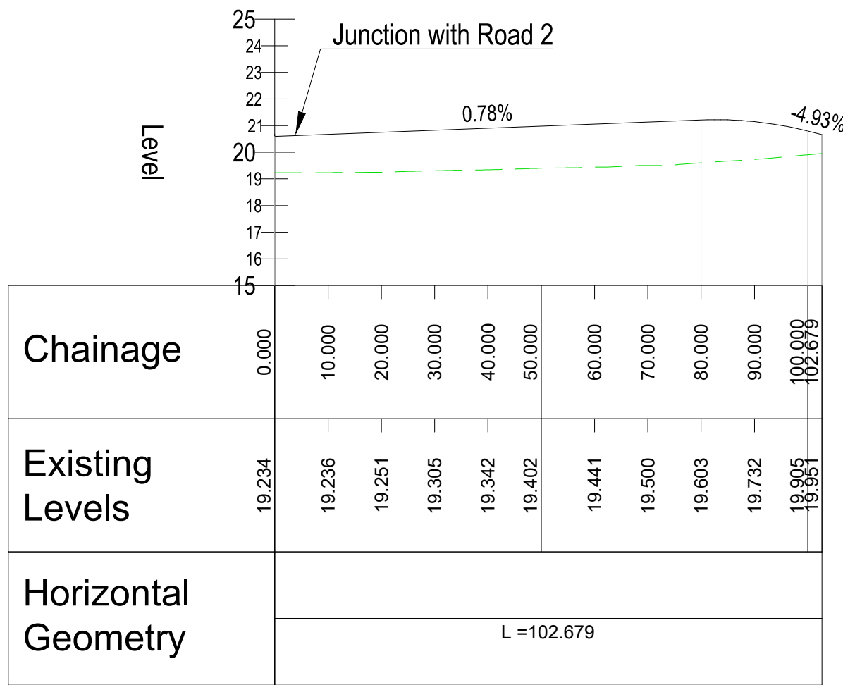
LONGSECTION - ALIGNMENT - PHASE 1 - ROAD 6 SCALE: H 1:1000,V 1:200. DATUM: 15.000
