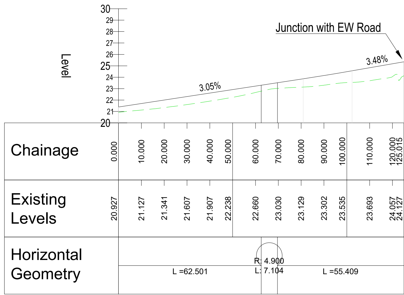
LONGSECTION - ALIGNMENT - PHASE 1 - ROAD 5 SCALE: H 1:1000,V 1:200. DATUM: 20.000
