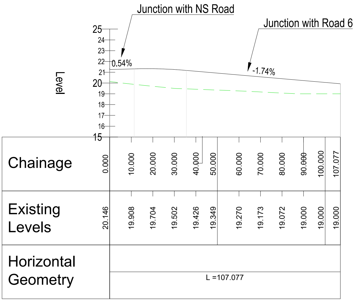
LONGSECTION - ALIGNMENT - PHASE 1 - ROAD 2 SCALE: H 1:1000,V 1:200. DATUM: 15.000
